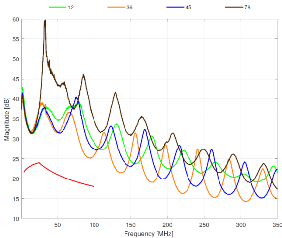
Typical Return Loss Cat.5e SF/UTP patch cord 2m
