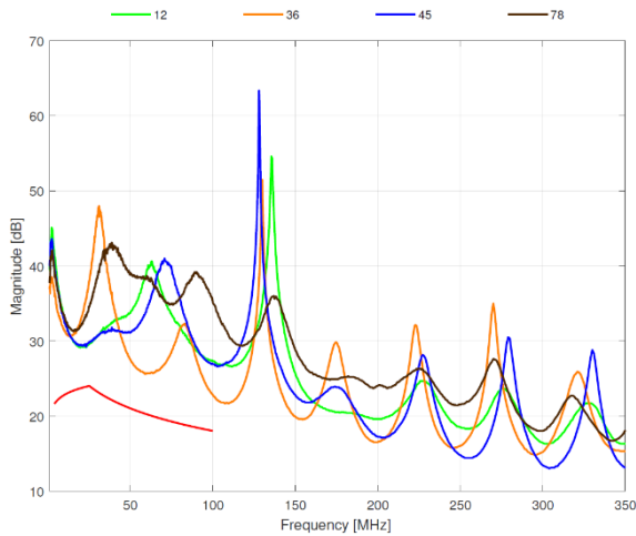
Typical Return Loss Cat.5e U/UTP patch cord 2m
