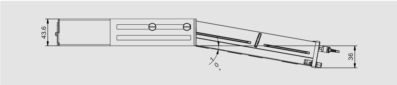
24x E-2000™ / SC / LC Duplex (Plastic front plate IntelliPhy ready)
