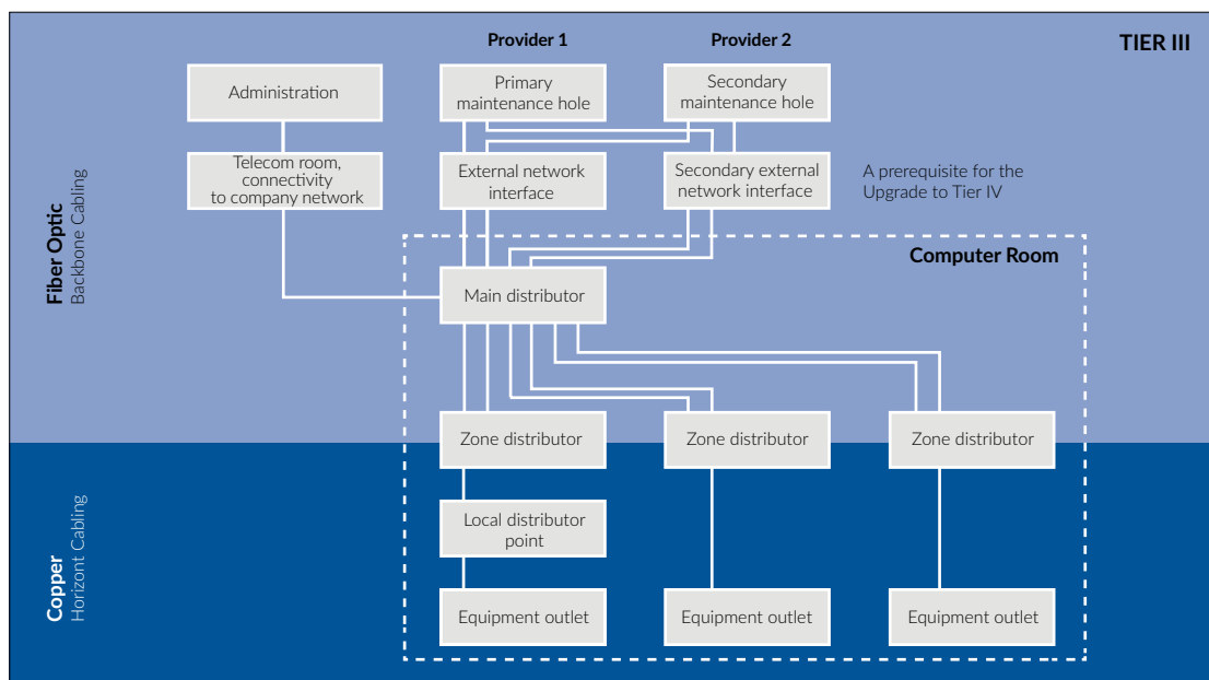
Principles of cabling TIER 3
