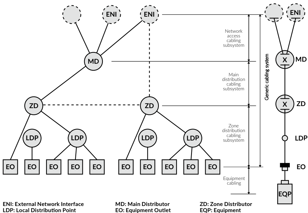
Describes the data center layout as well as its individual zones and their functions.
