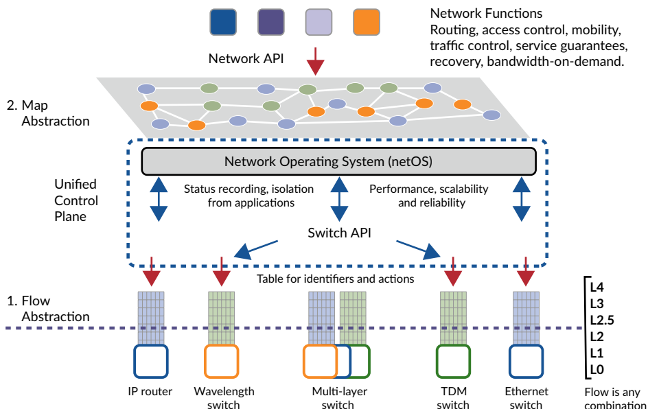
SDN-based unified control architecture
