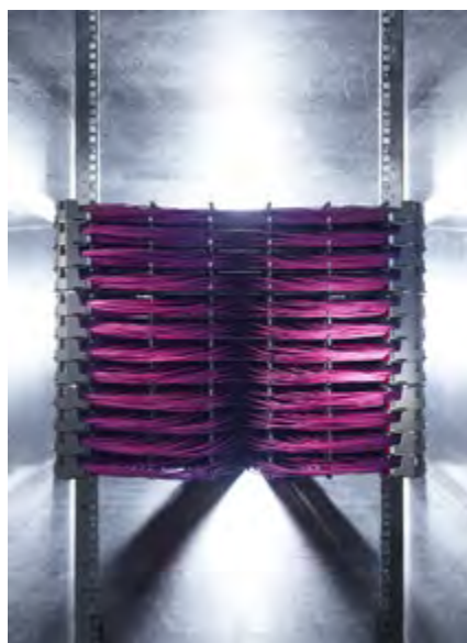
090.7602 Netscale 120 with the highest fiber density in the world
