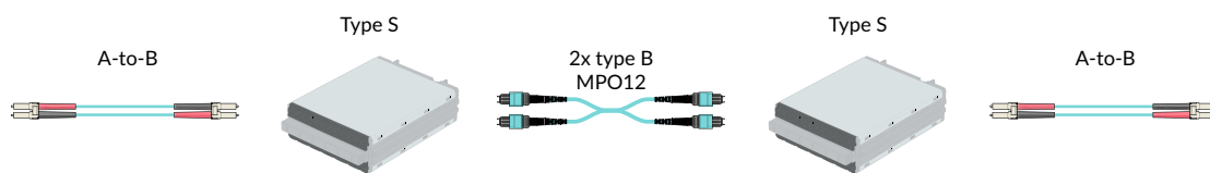
030.6130 Illustration of a link based on Type S modules before migration
