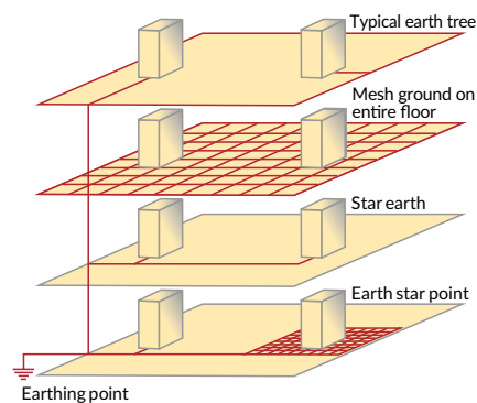
Earthing system as a tree structure
