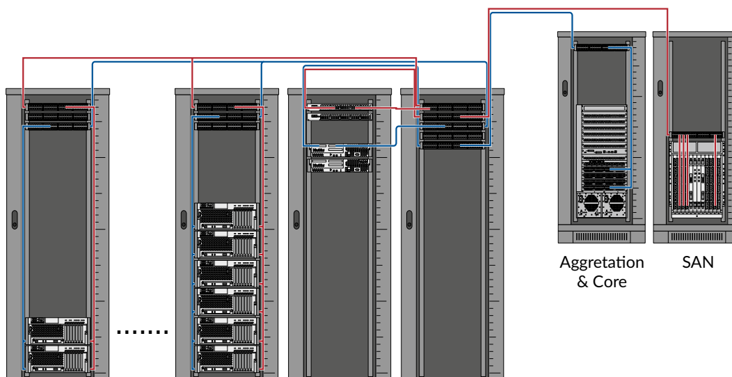
End of Row architecture
