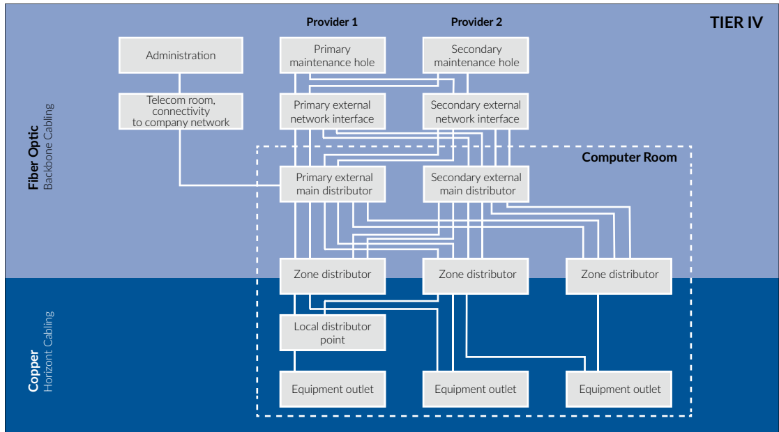
Principles of cabling TIER 4
