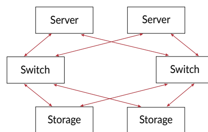
Example topology of a Fibre Channel switched fabric network
