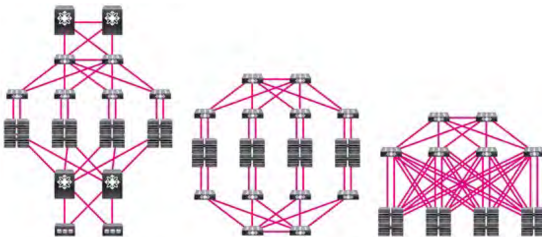
Left: classic design with Ethernet and fiber channel network. Center: SDS alternative for enterprise data centers with two separated Ethernet networks. Right: consolidated Ethernet network in which both data and storage traffic are distributed via the same switches.
