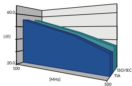
Connecting Hardware NEXT Values
