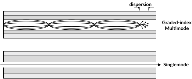
Illustrations of multimode (top) and singlemode (bottom) fiber
