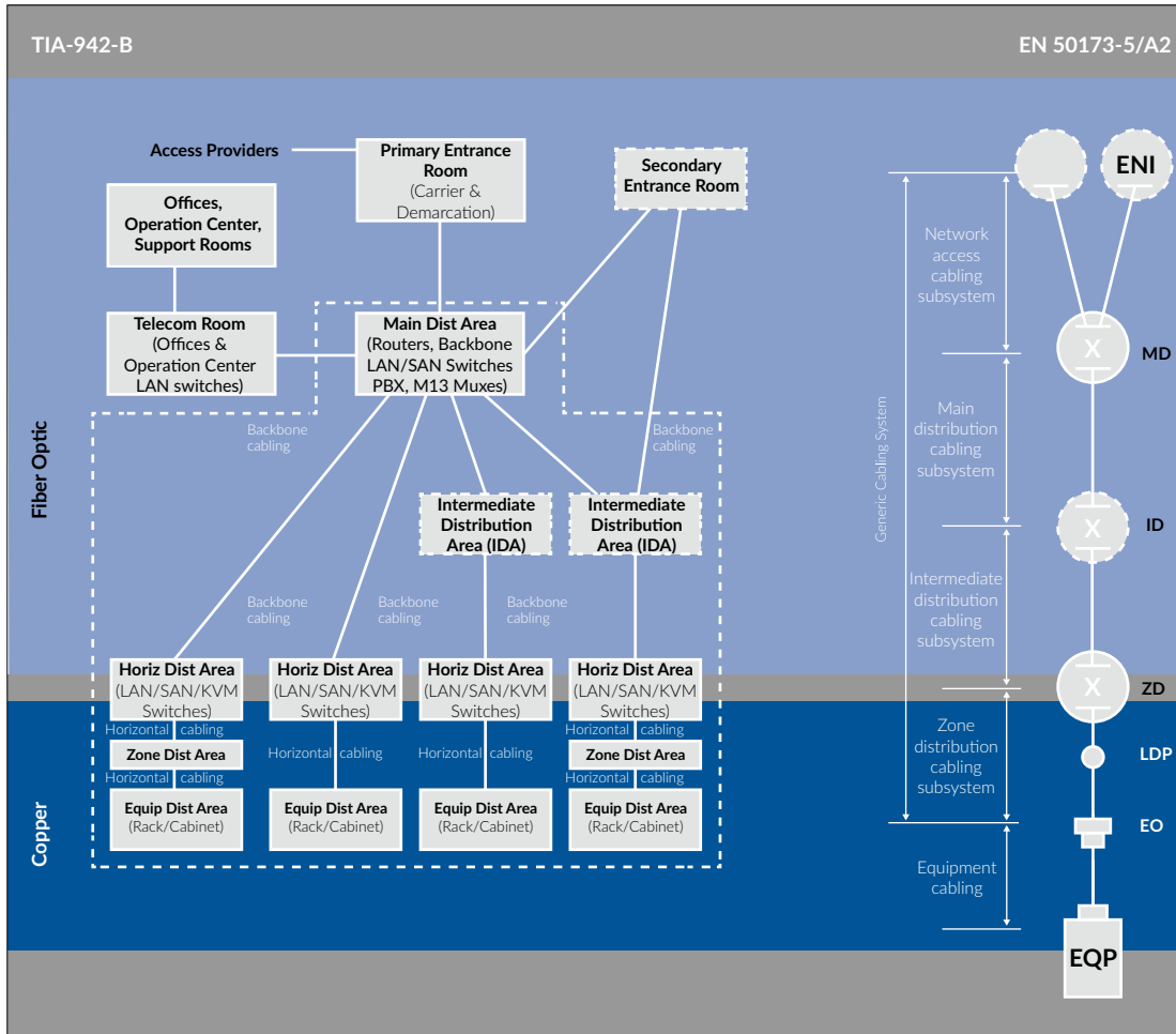
Comparison between TIA-942-B and EN 50173-5 cabling topology
