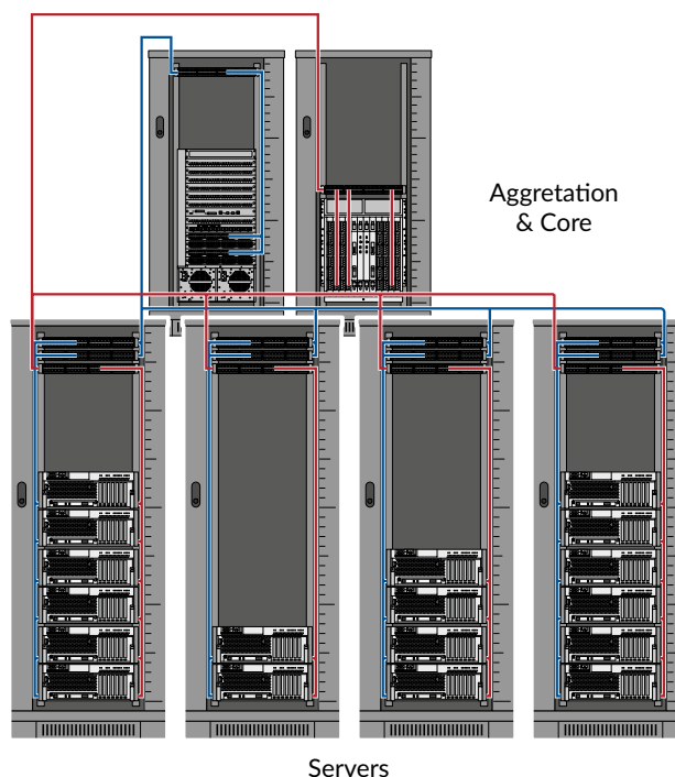
Centralized architecture
