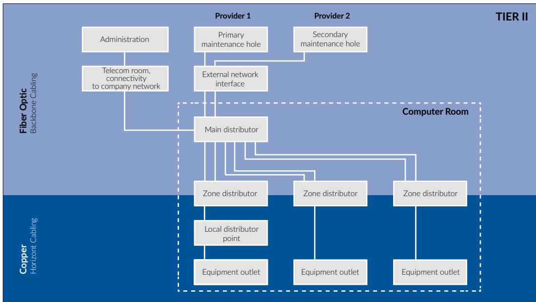
Principles of cabling TIER 2
