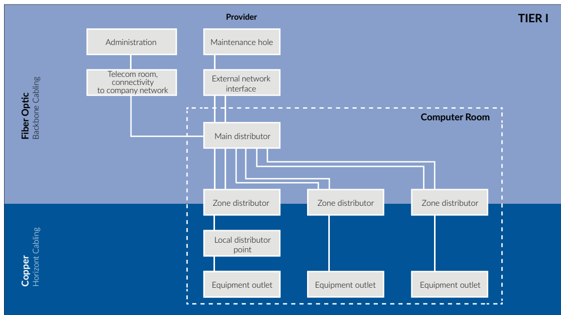
Principles of cabling TIER 1
