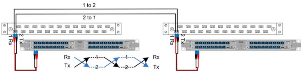
FO crossed backbone polarity
