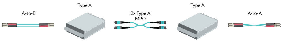
MPO polarity method A components
