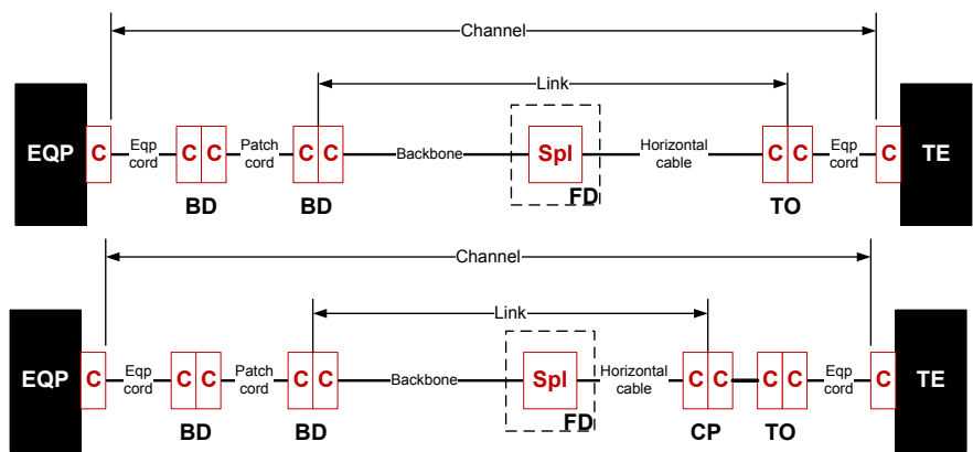
FO 4 connector combined splice
