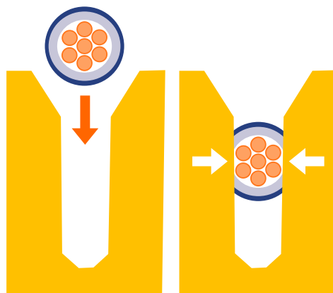
IDC contact
