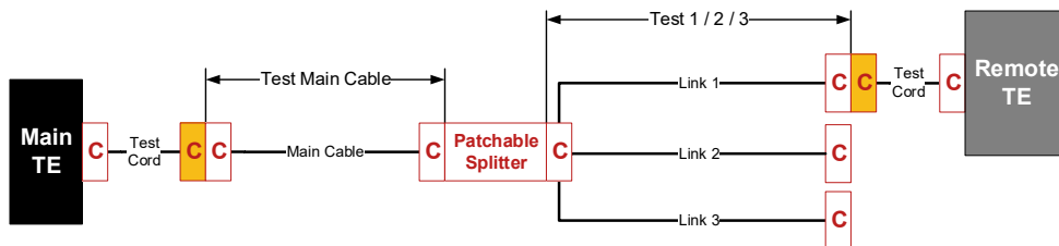
Direct test not possible through splitter
