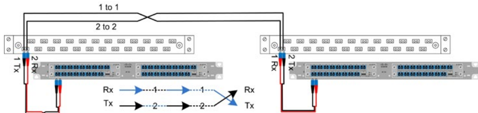
FO straight backbone polarity
