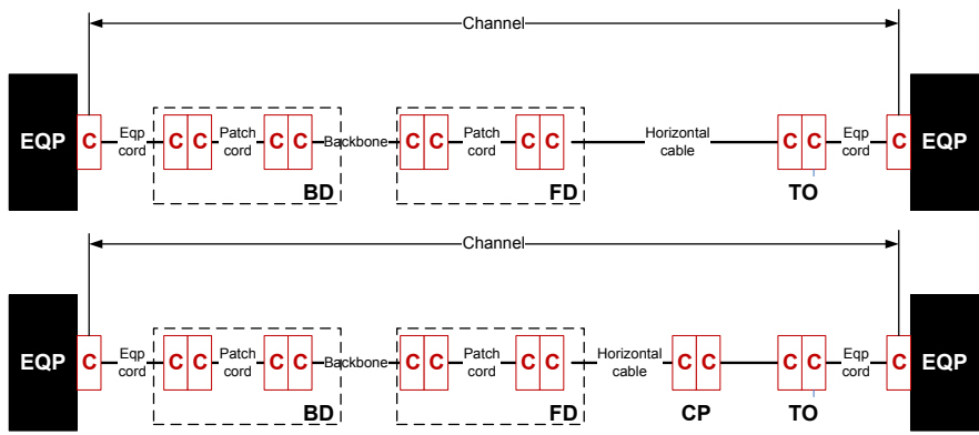
FO 5 connector direct combined
