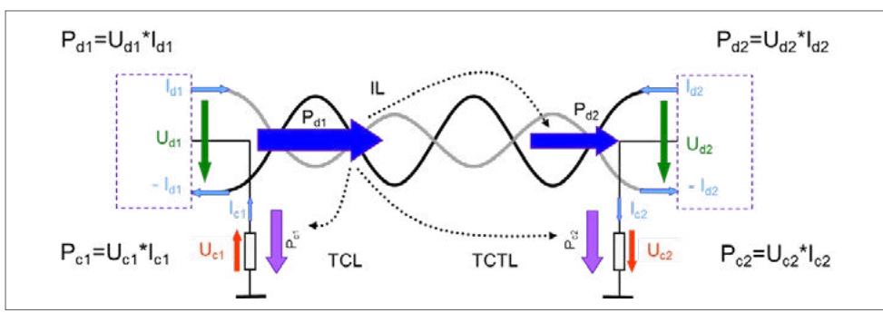
Influence TCL
