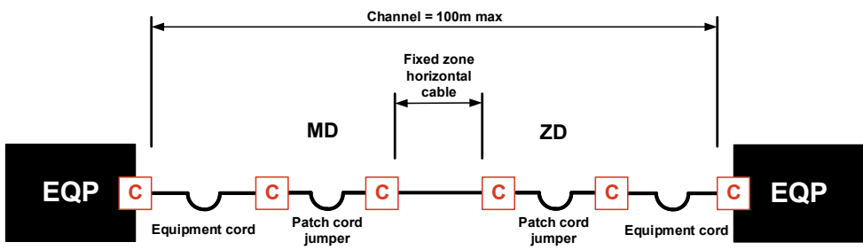
Cross-inter-cross connection model
