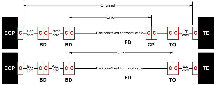
FO 3 Connector direct combined
