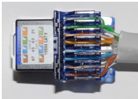
Câblage correct
