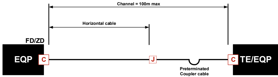
OC/DC 1-Connector Model MPTL with Cable-Coupler
